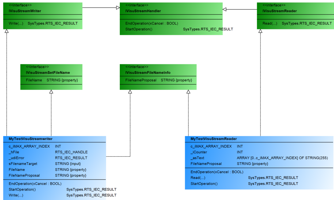
Class diagram VisuStreamReader / VisuStreamWriter
